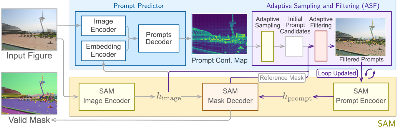
Figure 2: The architecture of our proposed AoP-SAM consists of two key components: the prompt predictor and the Adaptive Sampler and Filter (ASF) Module. The prompt predictor operates by taking the image input and the computed image embedding from SAM’s image encoder as inputs. Prompt predictor then generates a Prompt Confidence Map (PCM) that highlights potential regions for prompt candidates. During test-time, these candidates are adaptively sampled and filtered by ASF, predicting prompts that might lead to redundant masks based on the generated mask references. This process eliminates unnecessary prompts, ensuring that only the essential ones are used to generate the final mask results.
